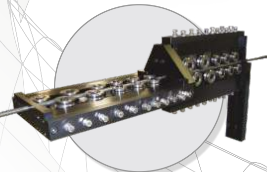
Dual Size Straightener Rollers for Wide Range of Wire Diameters
